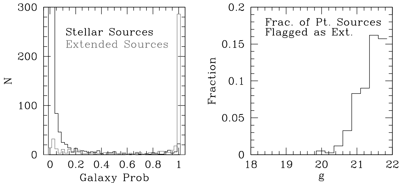
Figure 5. Left: Number of spectroscopically confirmed quasars classified by PHOTO as stellar ( black ) and as extended ( grey ) as a function of Bayesian galaxy probability (Scranton et al. 2002). Right: Fraction of point-like quasars (as determined by the Bayesian analysis) that are mis-classified by PHOTO as extended – as a function of magnitude.
